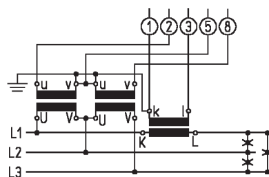
3-wire three-phase system - 3b, balanced load
