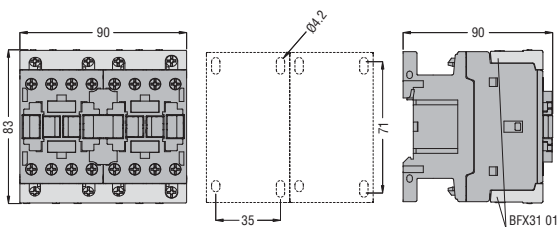
Starre Anschlüsse BFX31 01
